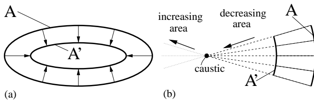
FIG. 4 Local definition of “inside”. (a) Ingoing rays perpendicular to a convex surface in a Euclidean geometry span decreasing area. This motivates the following local definition. (b) Inside is the direction in which the cross-sectional area decreases ( A' \leq A ). This criterion can be applied to light rays orthogonal to any surface. After light rays locally intersect, they begin to expand. Hence, light-sheets must be terminated at caustics.
