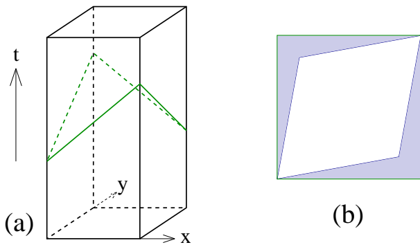
FIG. 9 (a) A square system in 2+1 dimensions, surrounded by a surface B of almost vanishing length A . (b) [Here the time dimension is projected out.] The light-sheet of B intersects only with a negligible (shaded) fraction of the system.
