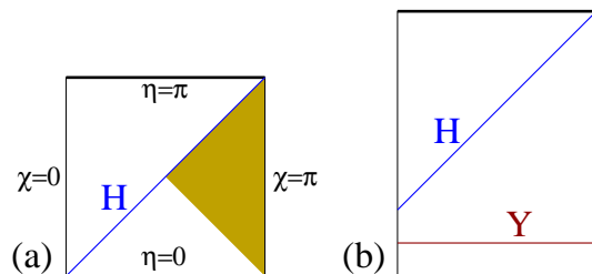
FIG. 10 (a) Penrose diagram for empty de Sitter space. H is the future event horizon of an observer on the south pole ( \chi = \pi ). The shaded region is the “southern diamond”. (b) Penrose diagram for a generic solution that asymptotes to de Sitter in the past and future ( dS^\pm ). The future event horizon has complete time slices in its past, such as Y .
