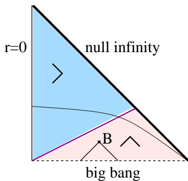
FIG. 5 Penrose diagram for an expanding universe (a flat or open FRW universe, see Sec. VII.A). The thin curve is a slice of constant time. Each point in the interior of the diagram represents a sphere. The wedges indicate light-sheet directions. The apparent horizon (shown here for equation of state p = \rho ) divides the normal spheres near the origin from the anti-trapped spheres near the big bang. The light-sheets of any sphere B can be represented by inspecting the wedge that characterizes the local domain and drawing lines away from the point representing B , in the direction of the wedge’s legs.
