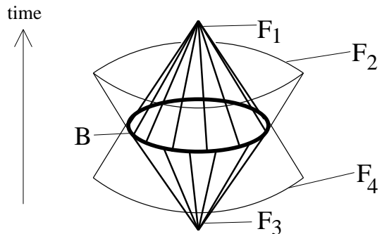
FIG. 3 The four null hypersurfaces orthogonal to a spherical surface B . The two cones F_1 , F_3 have negative expansion and hence correspond to light-sheets. The covariant entropy bound states that the entropy on each light-sheet will not exceed the area of B . The other two families of light rays, F_2 and F_4 , generate the skirts drawn in thin outline. Their cross-sectional area is increasing, so they are not light-sheets. The entropy of the skirts is not related to the area of B .— Compare this figure to Fig. 1.
