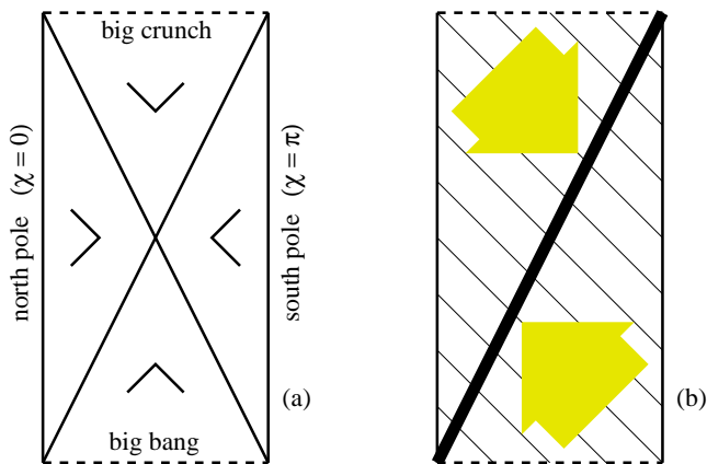
FIG. 7 (a) Penrose diagram for a closed FRW universe filled with pressureless dust. The three-sphere time slices are represented by horizontal lines (not shown). Two apparent horizons divide the diagram into four wedge domains: normal spheres are found near the poles, trapped (anti-trapped) spheres near the big bang (big crunch). (b) The construction of a global holographic screen (Sec. IX.C) proceeds by foliating the spacetime into a stack of light cones. The information on each slice can be stored on the maximal sphere, which lies on the apparent horizon.
