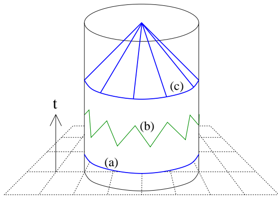
FIG. 2 The worldvolume of a ball of gas, with one spatial dimension suppressed. (a) A time slice in the rest frame of the system is shown as a flat plane. It intersects the boundary of system on a spherical surface, whose area exceeds the system’s entropy. (b) In a different coordinate system, however, a time slice intersects the boundary on Lorentz-contracted surfaces whose area can be made arbitrarily small. Thus the spacelike entropy bound is violated. (c) The light-sheet of a spherical surface is shown for later reference (Sec. V.C.1). Light-sheets of wiggly surfaces may not penetrate the entire system (Sec. VII.C).—The solid cylinder depicted here can also be used to illustrate the conformal shape of Anti-de Sitter space (Sec. IX.B).
